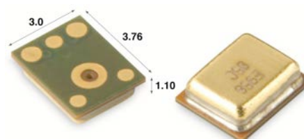
Figure 4. MEMS microphone with dimensions in millimeters.
