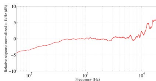
Figure 5. PCB mounted MEMS microphone frequency response normalized at 1kHz.
