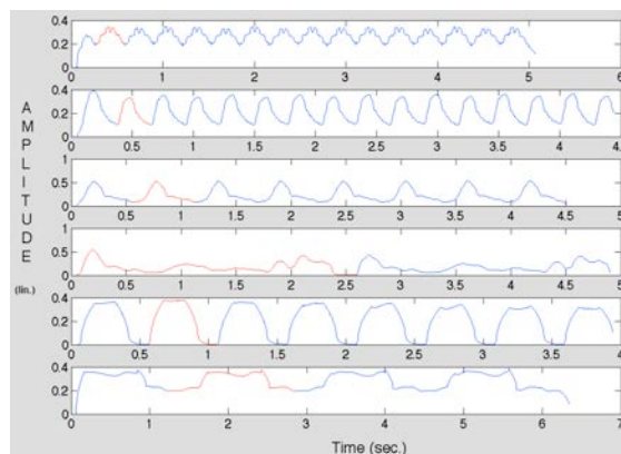
Figure 8. Six car alarm inter-onset intervals (IOI's). For each profile, the blue line represents the whole profile and the red line represents the elementary profile used for computing standard values of IOI's.
