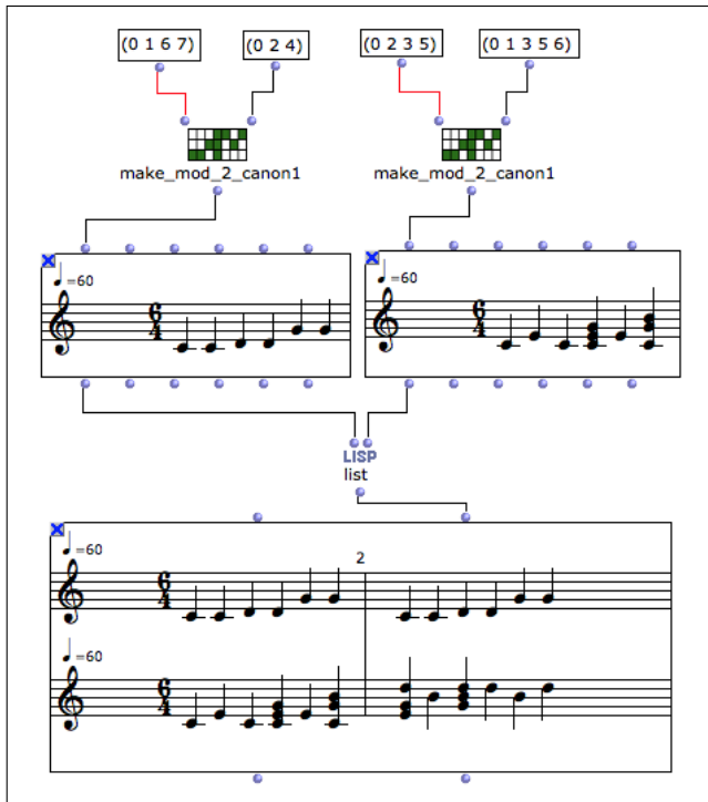
Figure 3. An OpenMusic patch representing two RT_2C of \mathbb{Z}_{12} . The upper one is not Vuzza whilst the second one is.
