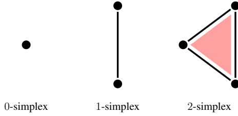
Figure 1. Some simplices.
