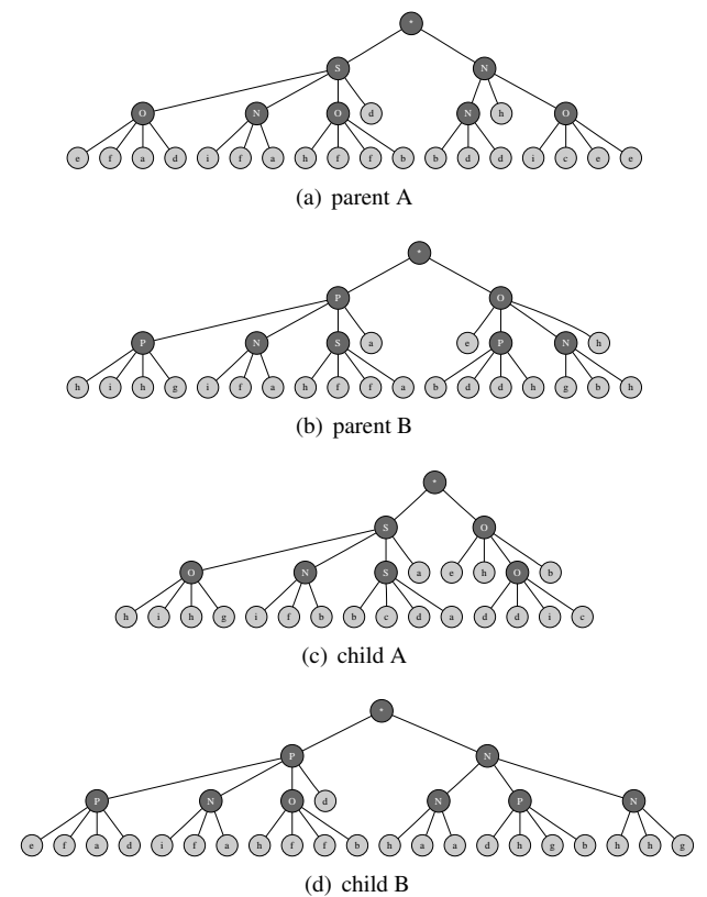
Figure 6. Recombination
