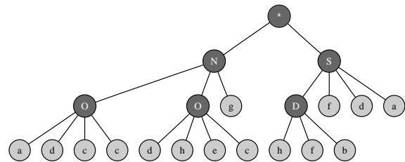
Figure 3. Expression tree of a multigenic chromosome with multiplication function serving as a linker.
