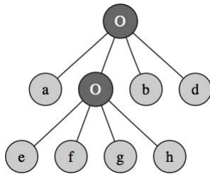
Figure 2. Decoded expression tree of phase modulation as a graph of sine oscillators. Sine oscillators are designated by capital O and terminals by lower case letters
