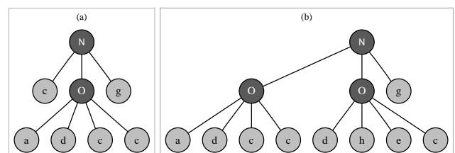
Figure 4. Single-point mutation. A terminal in (a) changes into a sine oscillator function in (b)
