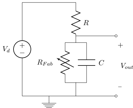
Figure 3. Passive circuit of the pressure sensor. In this diagram, R_{Fab} is the variable resistance of the fabric.
