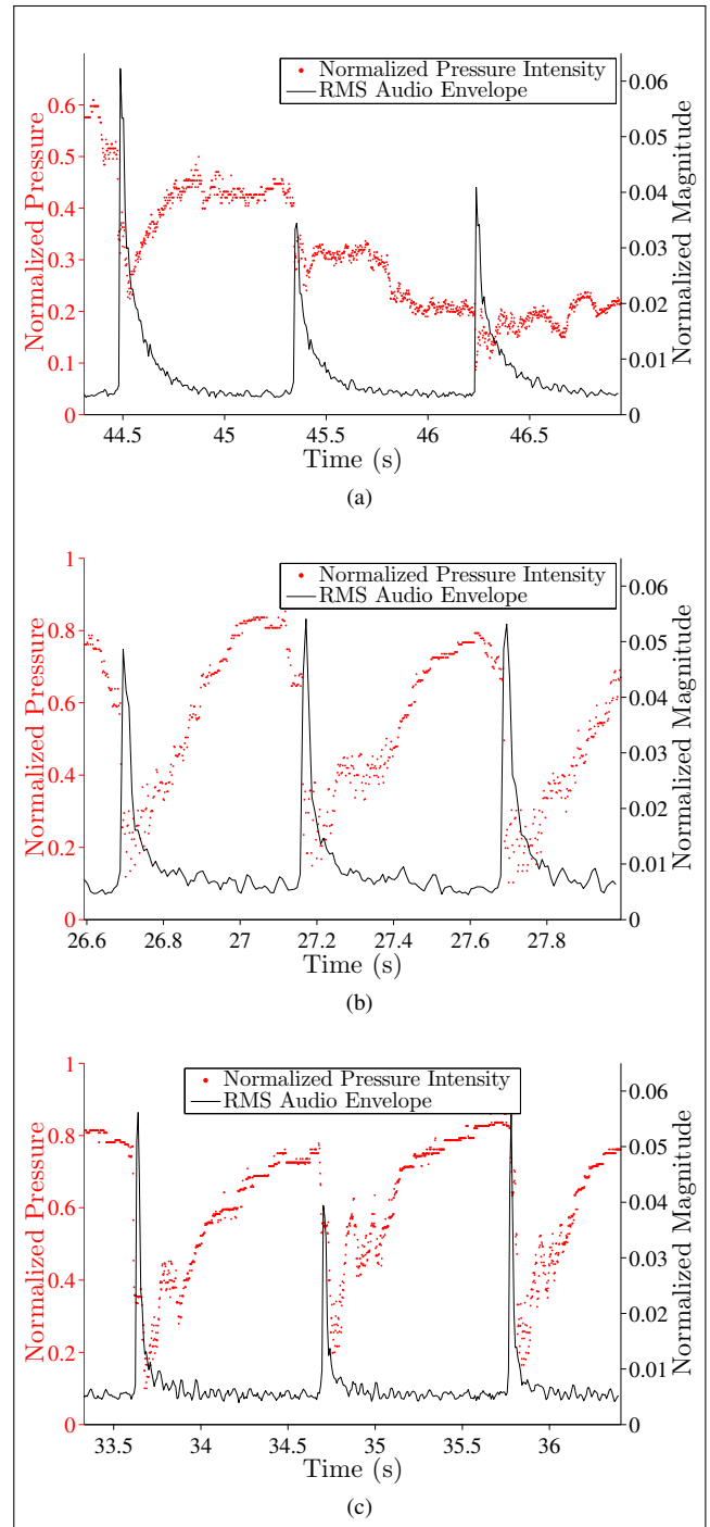
Figure 10. Normalized pressure intensity over time on the second area of the sensor with its associated audio RMS envelope for: (a) downward picking, (b) upward picking, (c) alternate picking.
