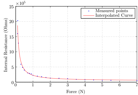
Figure 4. Measured response of the internal resistance of the piezoresistive fabric to an applied force on the pressure sensor.
