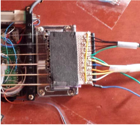
Figure 2. First attempt to sense the guitar thanks to a pressure sensor array attached right onto the guitar bridge.
