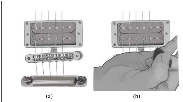
Figure 5. Positioning of the hand when the guitarist does palm muting: (a) palm muting area without the hand, (b) palm muting applied by the side of the hand. Therefore, the area between the bridge and the bridge pickup must be sensed to measure this technique.
