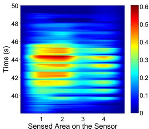
Figure 9. Measured response of the sensor (x axis) to the rolling gesture of the palm over time (y axis). The intensity of the colors represents the intensity of the normalized pressure on the sensor.
