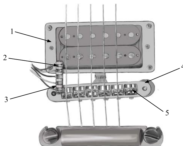
Figure 1. Diagram of the developed pressure sensor and its disposition: (1) Pickup; (2) Conductive band; (3) Fret (used as a sensor support); (4) Bridge; (5) Saddle.
