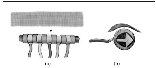
Figure 8. Prototype of one pressure sensor to mount along the string: (a) Profile view, (b) Front view. We see the fabric laying on the top of the conductive rings, whose are connected to wires.
