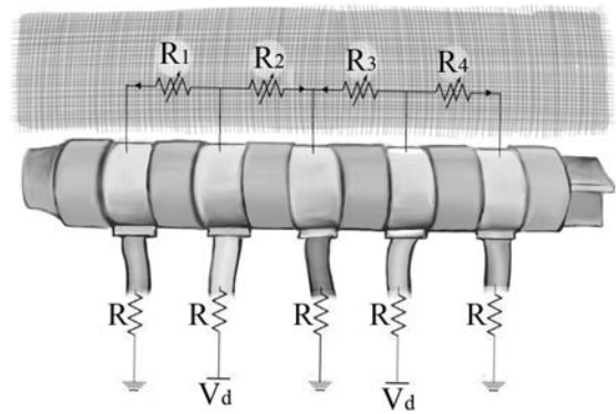
Figure 7. Equivalent electrical network of the pressure sensor, where V_d is the power voltage, the fabric, at the top, acts like variable resistors between each conductive ring. The resistors R are pull-up and pull-down resistors that allows the measure of the variable resistors and maintain a similar dynamic for each area.
