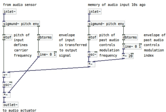
Figure 3. Signal processing Pd abstraction used in this example
