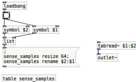
Figure 5. Pd abstraction for receiving a signal from an audio sensor
