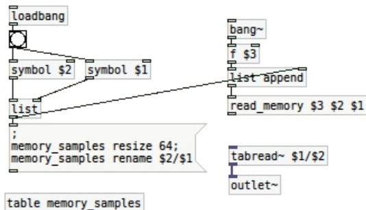
Figure 6. Pd abstraction for reading from memories of an agent
