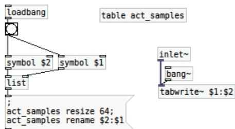
Figure 4. Pd abstraction for writing a signal to an actuator
